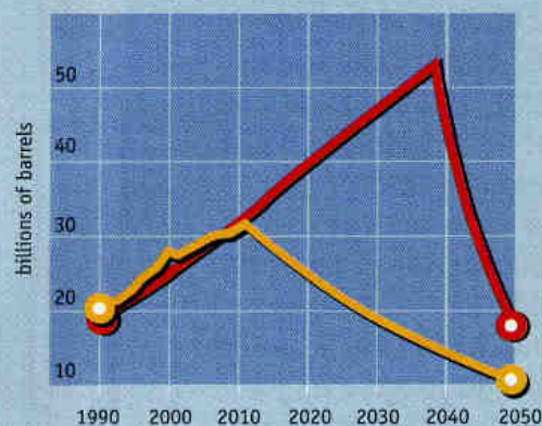
Annual oil production
