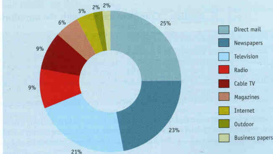
US advertising spend (billion $)
